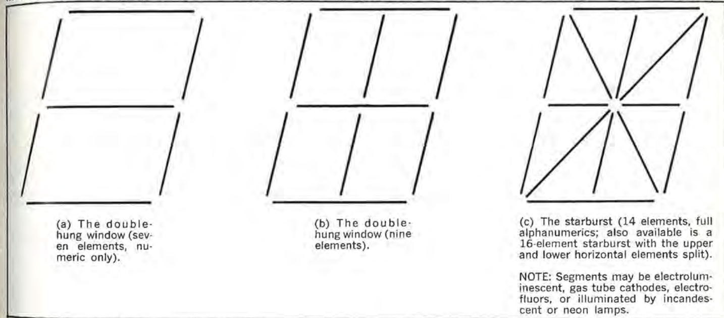
FIGURE 6: Segmented character formats.
